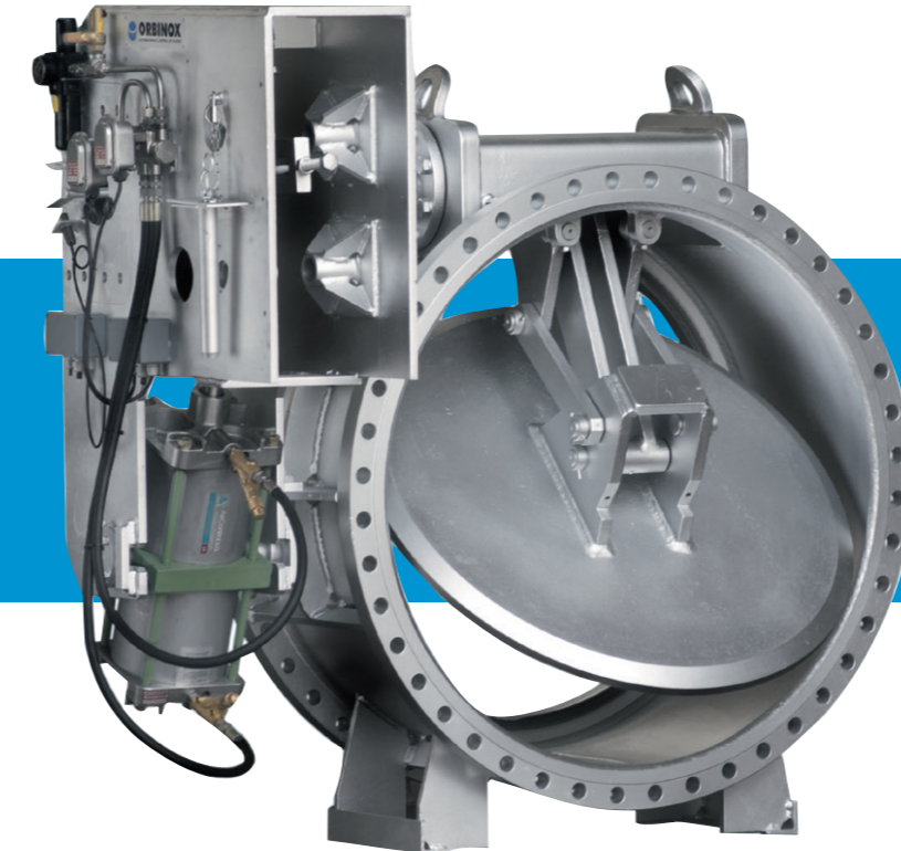
MP Three-lever valve
